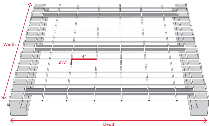
STEP CHANNEL
